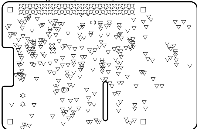
Drill Drawing View (Scale 1:1)
